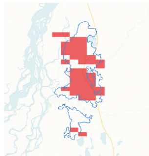
MODIS burnt area
