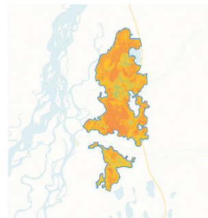
Landsat-Liberty burnt area
