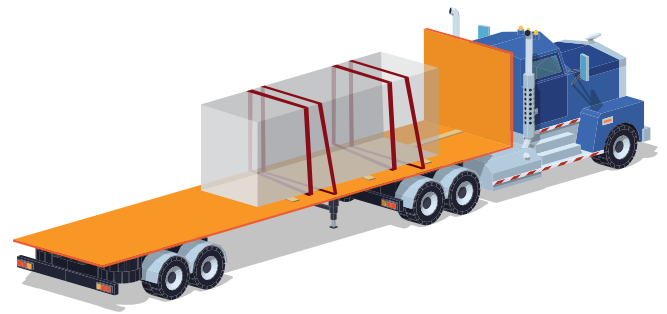
Loop lashing
