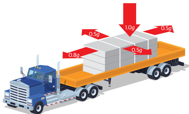
Forces at play in cargo under acceleration
