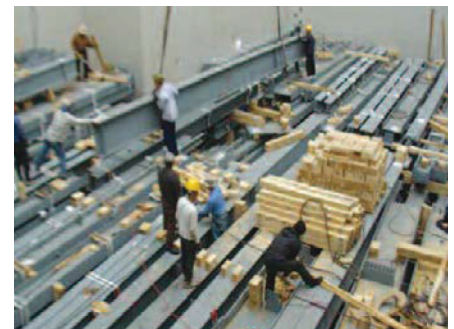
Well-stowed structural steel (fore and aft direction), with adequate dunnage between tiers
